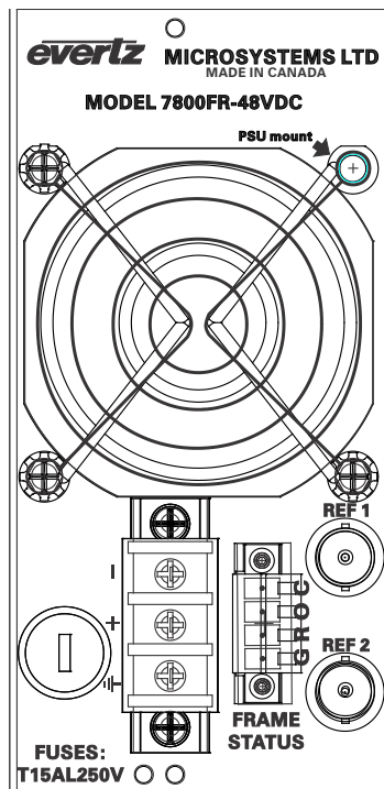
Figure 0-2: 7800FR-C-48VDC Rear Panel
