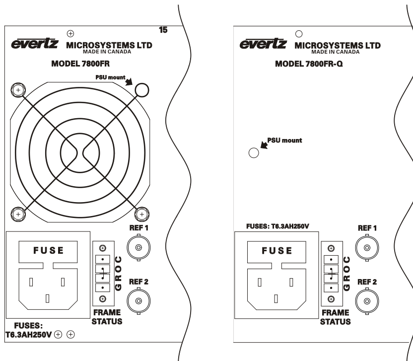
Figure 0-1: AC Powered Frames Rear Panel
