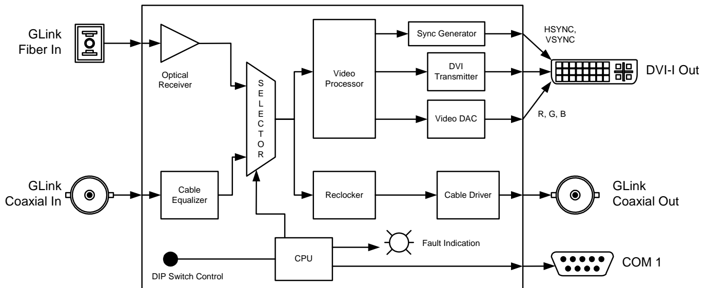
Figure 1-1: 2430GDAC Block Diagram
