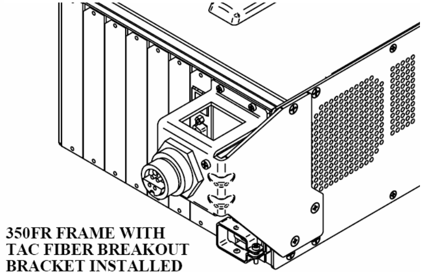
Figure 5-4: Fiber Breakout Bracket Contents and Final Assembly
