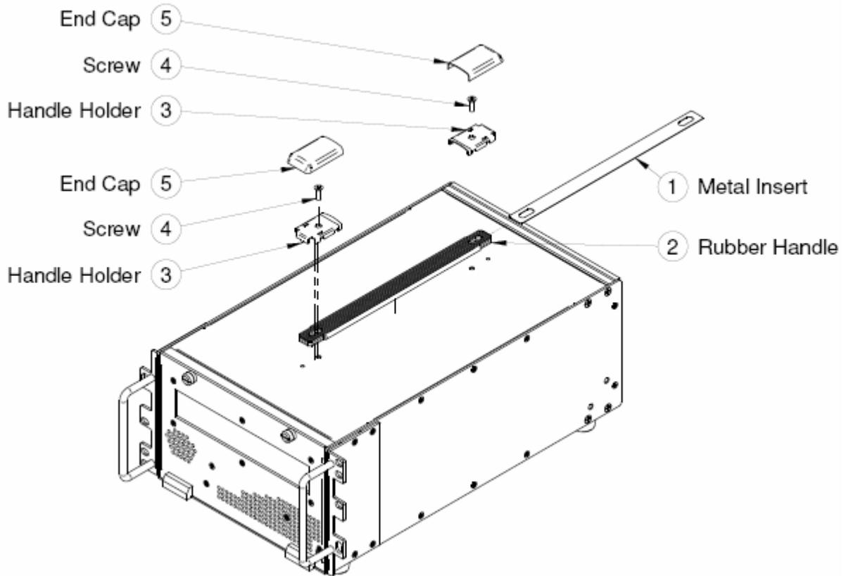
Figure 5-2: Portable Carry Handle Installation
