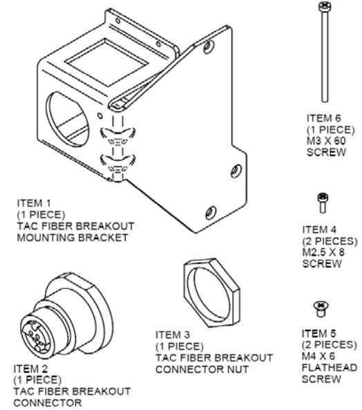
Figure 5-4: Fiber Breakout Bracket Contents and Final Assembly
