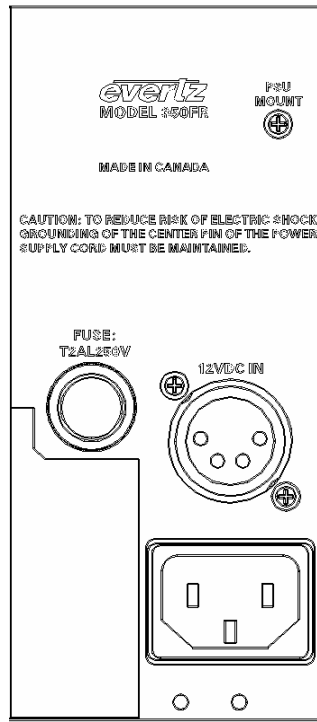
Figure 2-2: 350FR Power Supply Rear Panel
