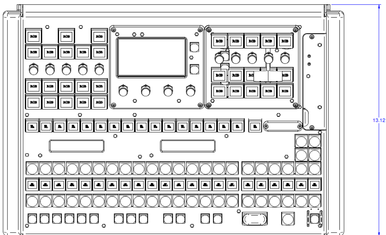
Figure 4-3: EMC-DCP Top View
