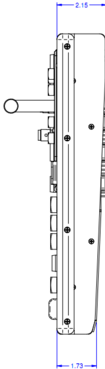
Figure 4-5: EMC-DCP Side View Without Desktop Mount
