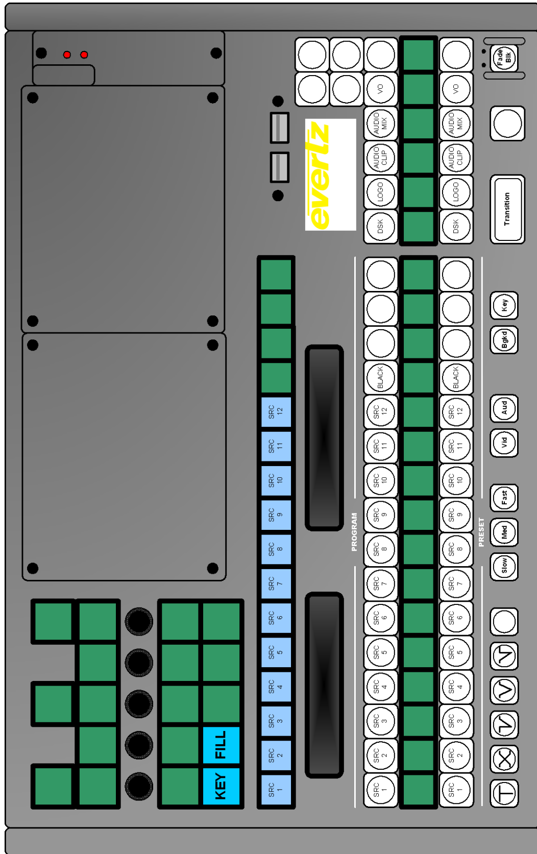
Figure 3-16: EMC-DCP Layout for Mini Master Control
