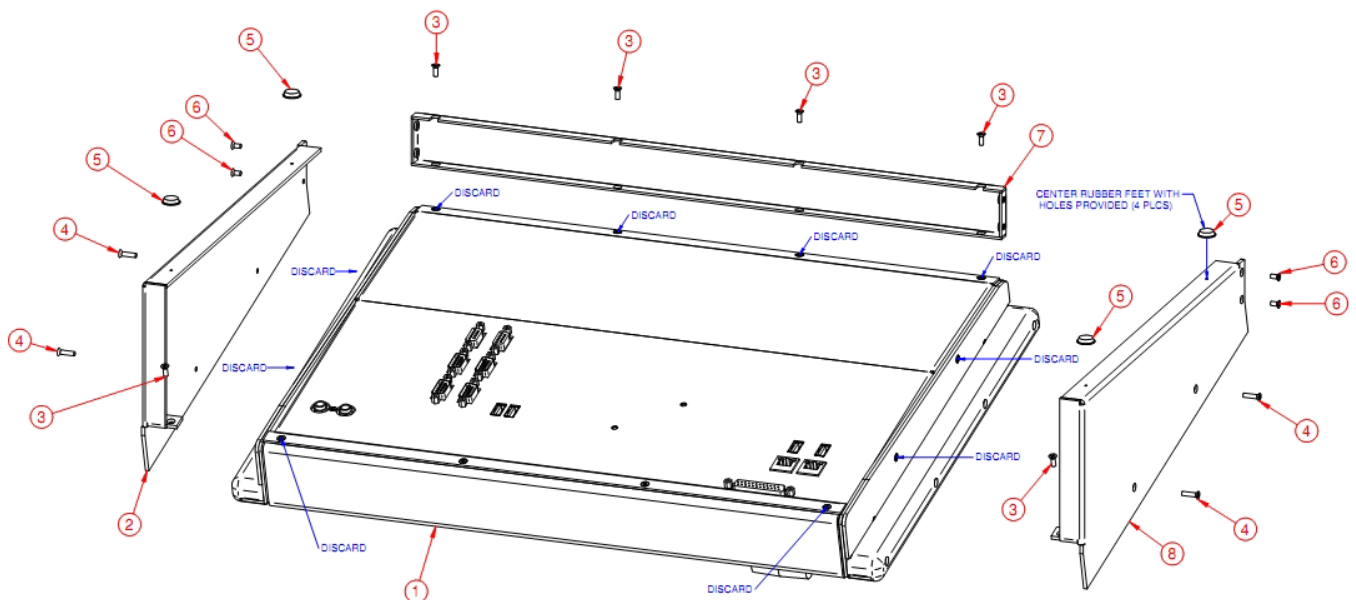
Figure 5-1: Pre-Assembled Unit
