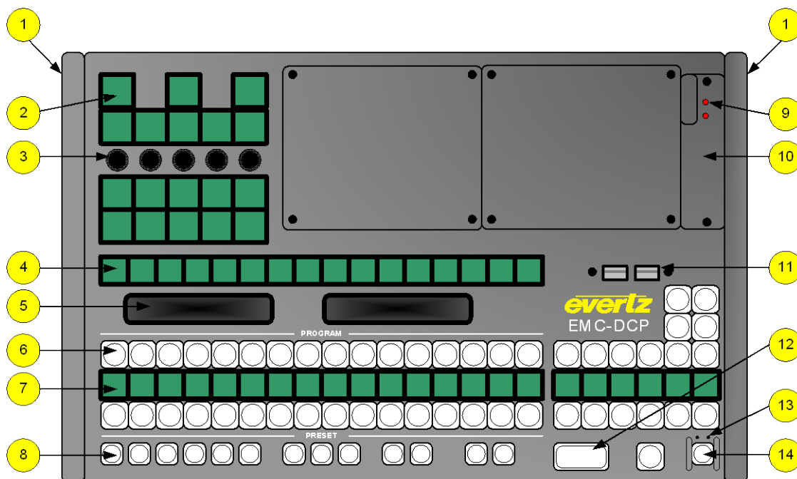
Figure 3-4: EMC-DCP Top Panel
