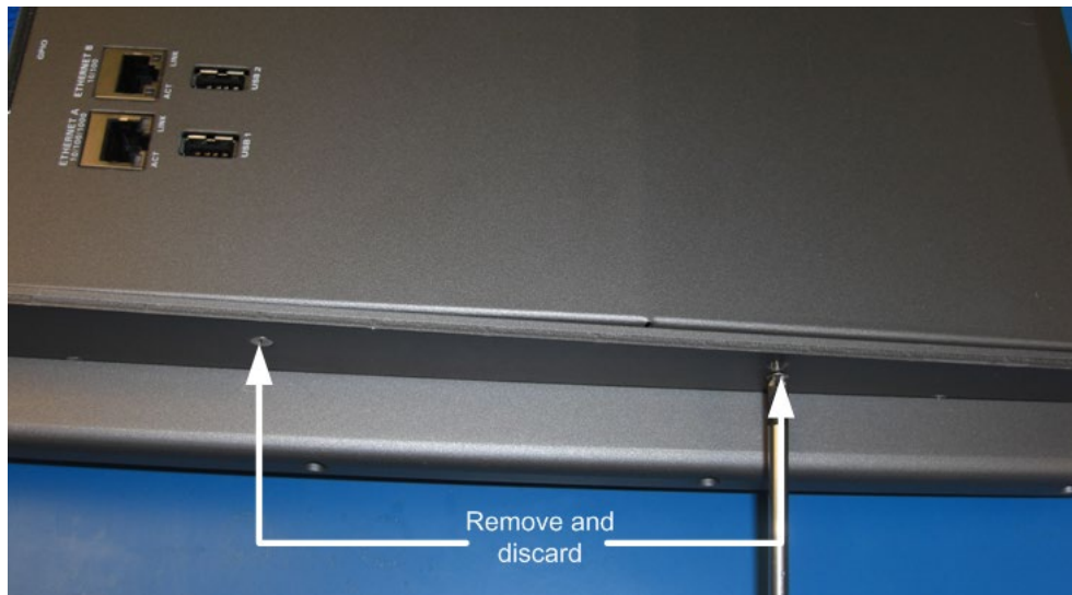
Figure 5-2: Side Screws
