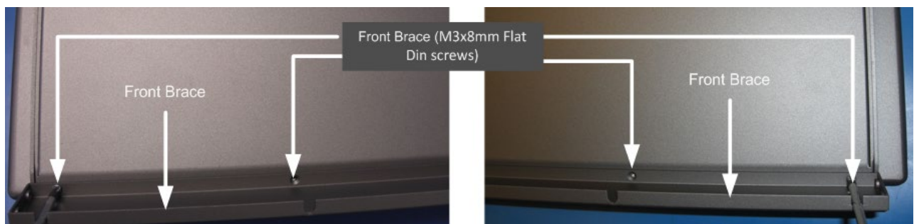
Figure 5-5: Front Brace
