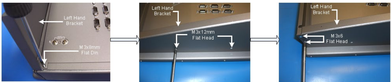
Figure 5-6: Bracket Assembly
