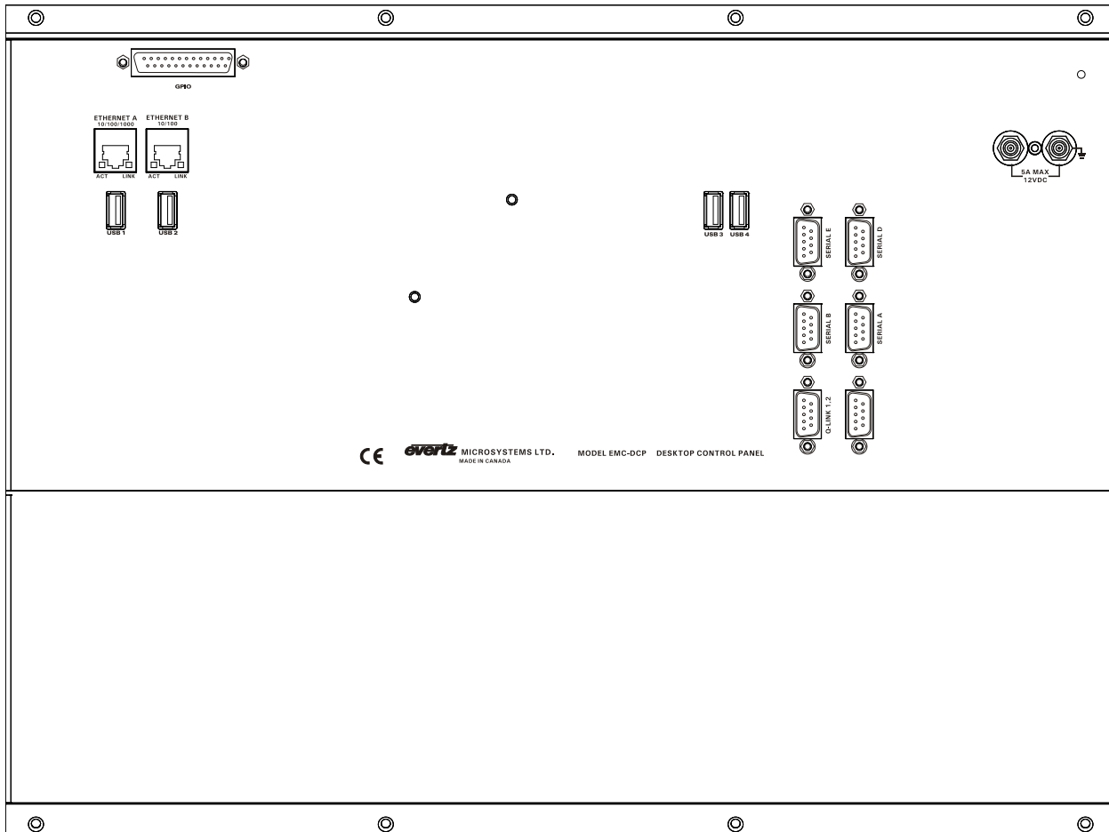
Figure 3-5: EMC-DCP – Inputs and Outputs
