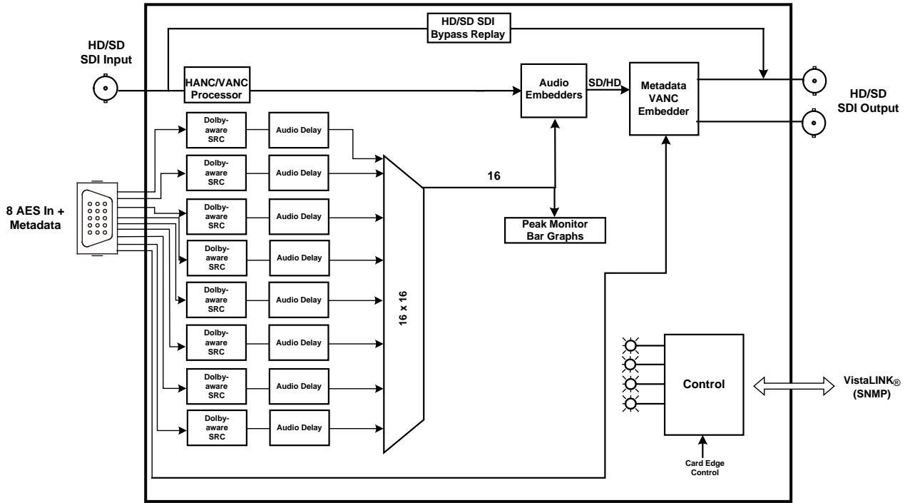
Figure 1-1: 7721AE8-HD Block Diagram
